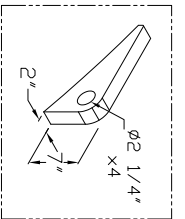
LIFTING LUG DETAIL
